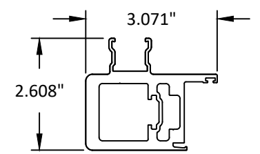
10 OUTSIDE CORNER ASTRAGAL STILE/SASH 6063-T5
