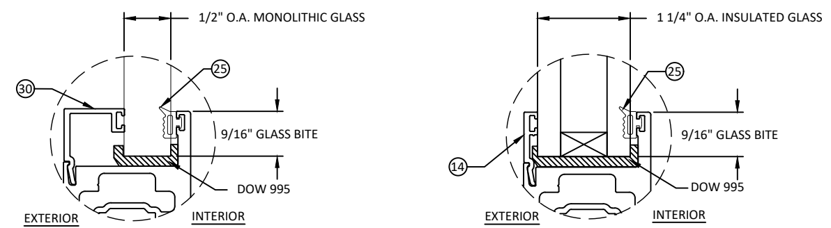
GLAZING DETAIL 1
