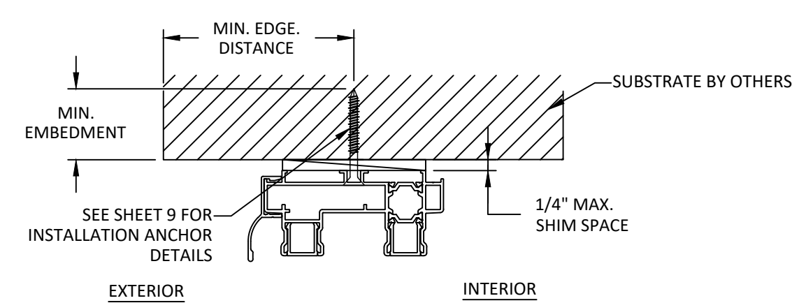
B 8 ANCHOR DETAIL THROUGH FRAME INSTALLATION (HEAD) 2 TRACKS
