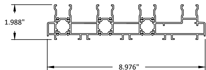
34 INSIDE CORNER ASTRAGAL STILE/SASH 6063-T5
