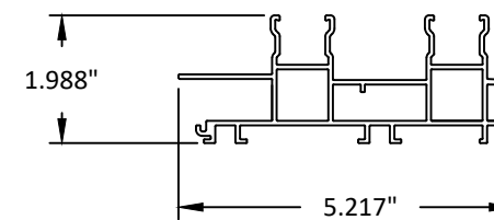
33 2 TRACK JAMB/HEAD/SILL (ADD-ON) 6063-T5
