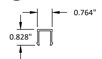
12 JAMB/HEADER TRIM 6063-T5
